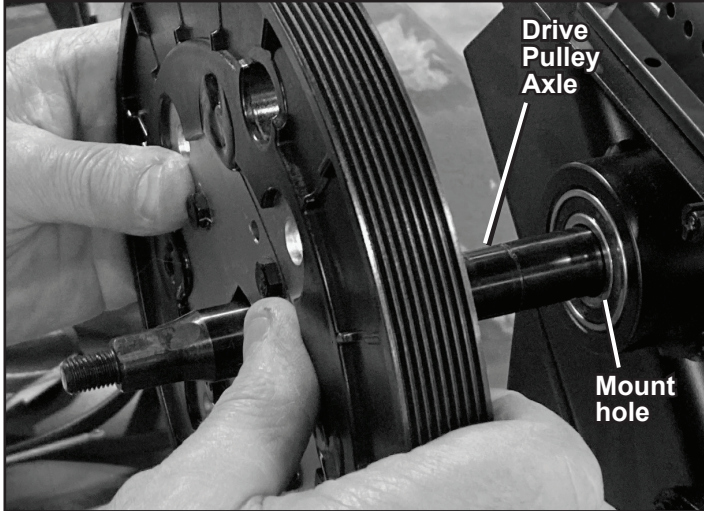
Left side — Align drive pulley axle with mount hole in frame
